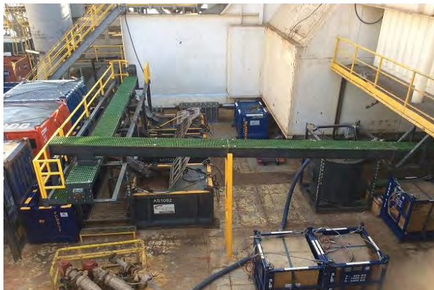
ANSS DWM Skips and Auger arranged aboard the Ensco 101
